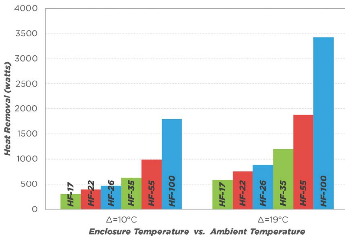
Heat Removal at Recommended \Delta T
